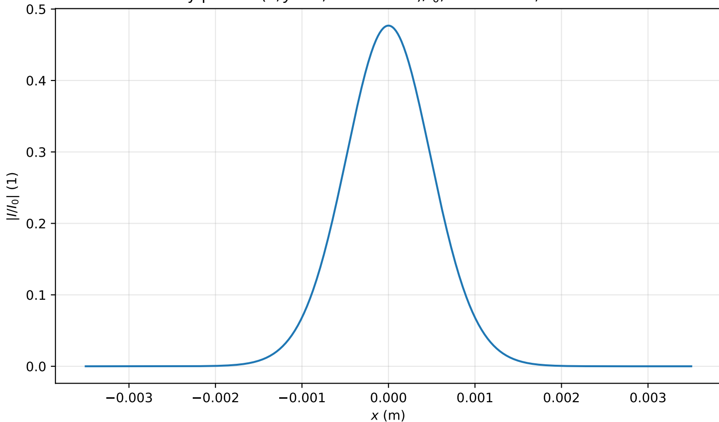
Intensity profile I(x, y = 0, z = 2.468m)/I_0 , P_{in}=0.2P_{cr} , artificial time
